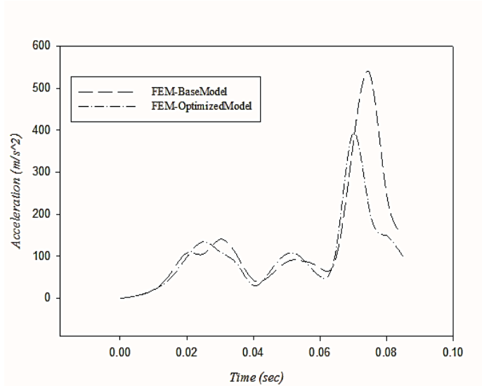
Fig24. A comparison between time histories of accelerations of the occupant’s body, for the original and optimized designs
